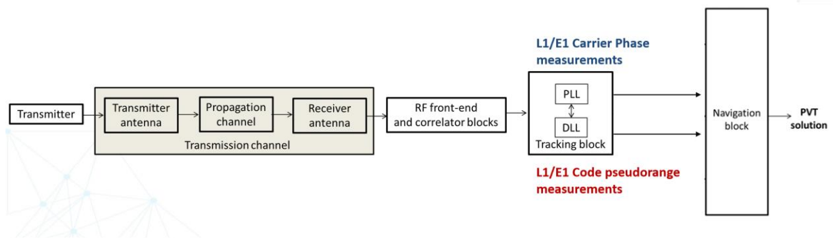
Figure 2-7 GNSS receiver architecture (Single-frequency)
