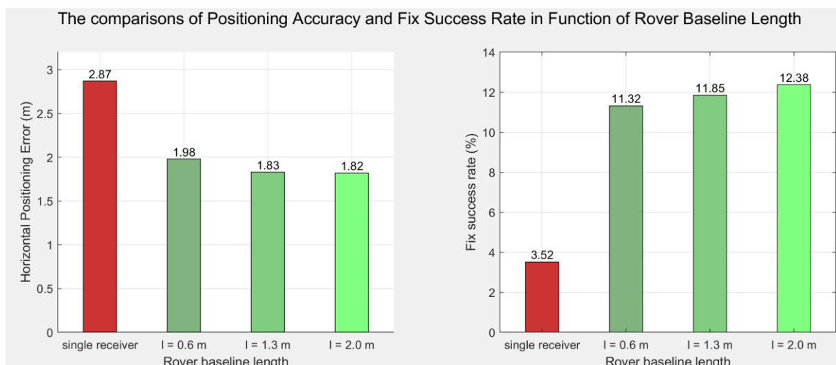
Figure 6-53 Comparisons of Positioning Accuracy and Fix Success Rate w.r.t Rover Baseline Length (Dataset3- GPS/GALILEO)
