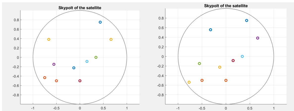
Figure 5-18 Considered GPS/Galileo satellite geometry with N_{sat}=10 (left) and N_{sat}=12 (right)
