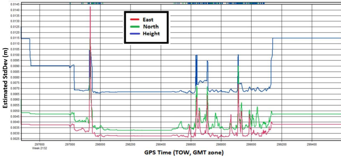
Figure 6-13 Estimated position standard deviation in ENU frame of the reference solution for dataset 2
