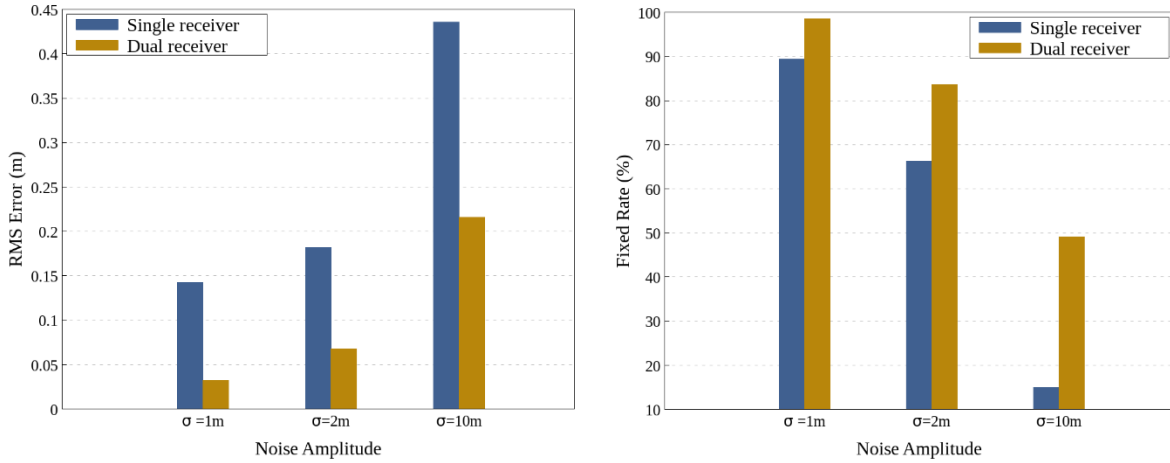
Figure 5-33 The comparisons of Position accuracy and fix success rate under different measurement noise (0 baseline)
