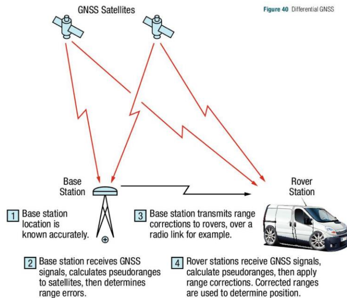
Figure 3-1 Differential GNSS(DGNSS) [43].
