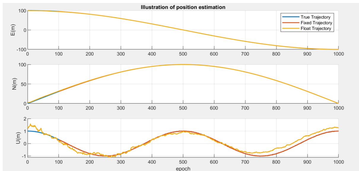
Figure 5-6 Illustration of the position estimation
