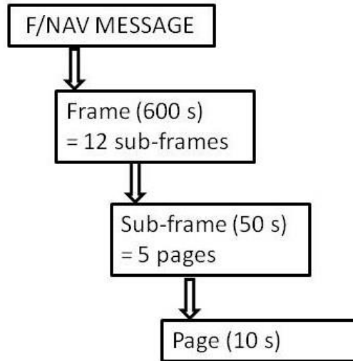
Figure 2-4: F/NAV message structure [18]
