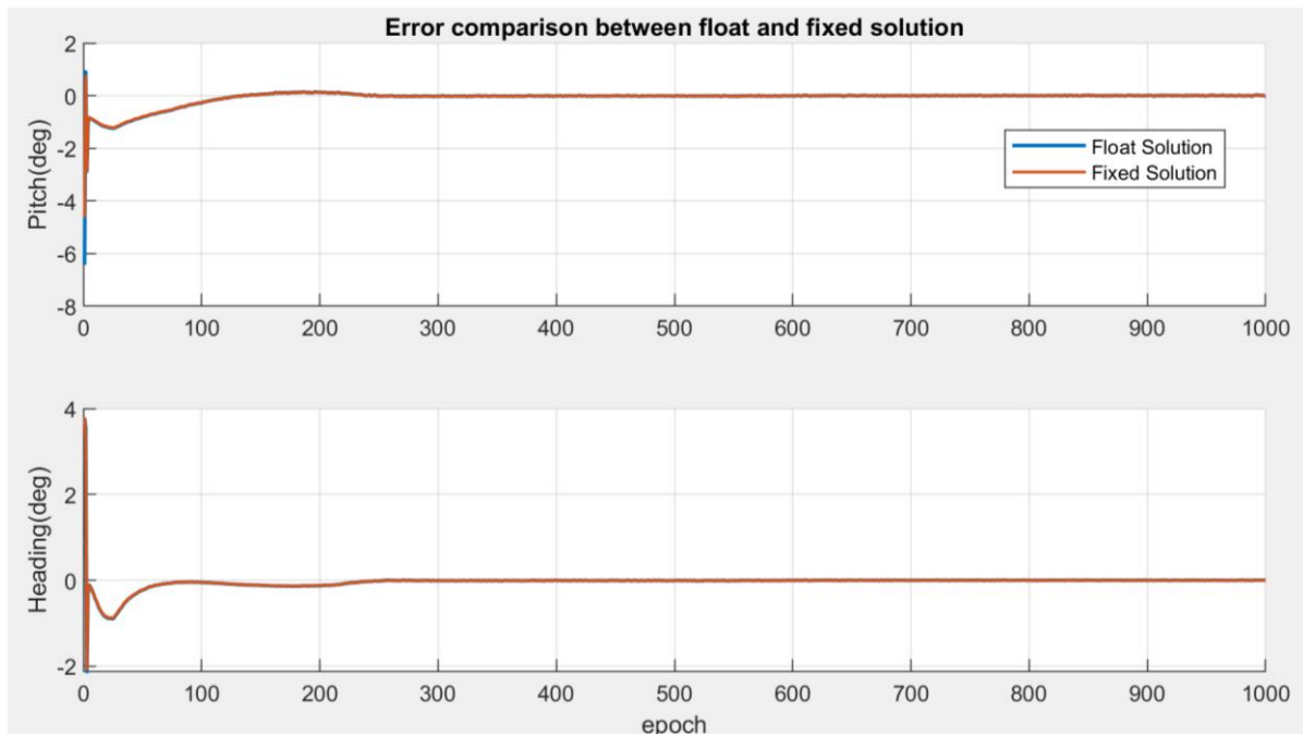
Figure 5-11 Error comparison between float and fixed solution for attitude estimation
