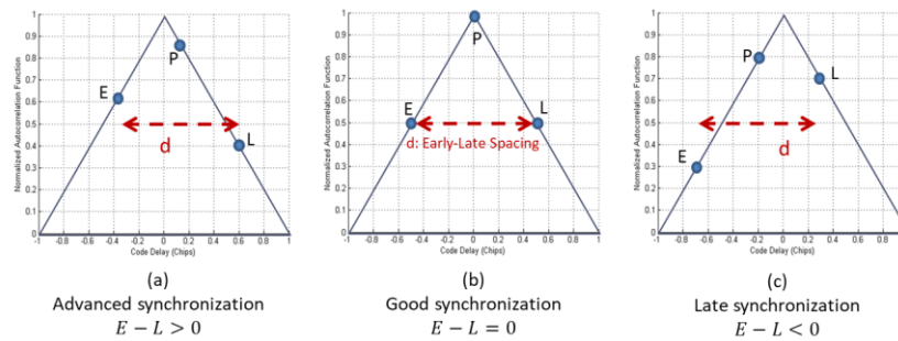
Figure 2.25 – DLL principle
