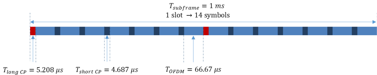
Figure 3.25 – Slot structure
