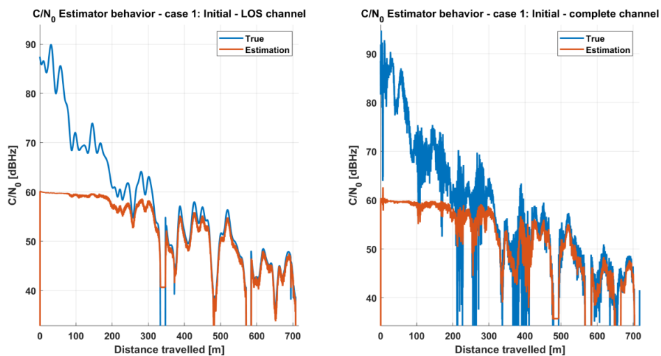
Figure 5.26 – Estimator behavior – Case 1
