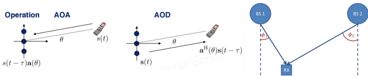
Figure 3.9 – AoA and AoD principles
