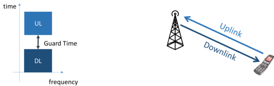
Figure 3.22 – Time Division Duplex principle
