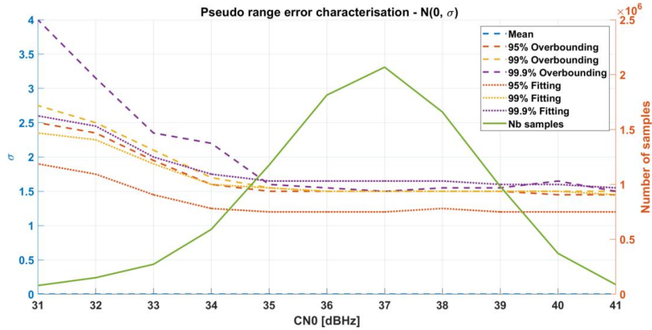
Figure 6.34 – GNSS characterization
