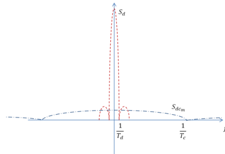
Figure 2.10 – Comparison of S_d and S_{dc_m}
