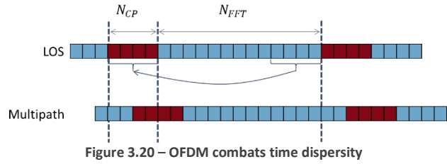
Figure 3.20 – OFDM combats time dispersity
