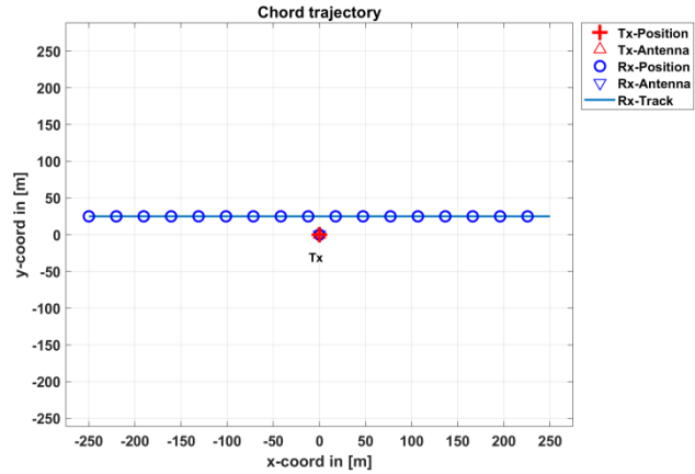
Figure 6.13 – Chord trajectory
