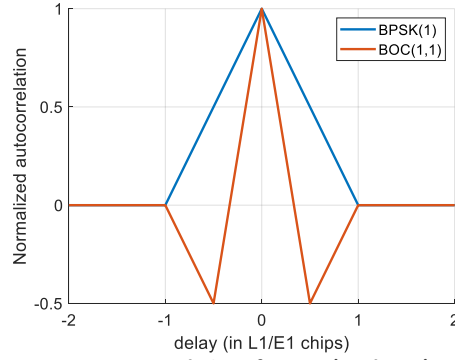
Figure 2.15 – Autocorrelation of BPSK(1) and BOC(1,1) signals
