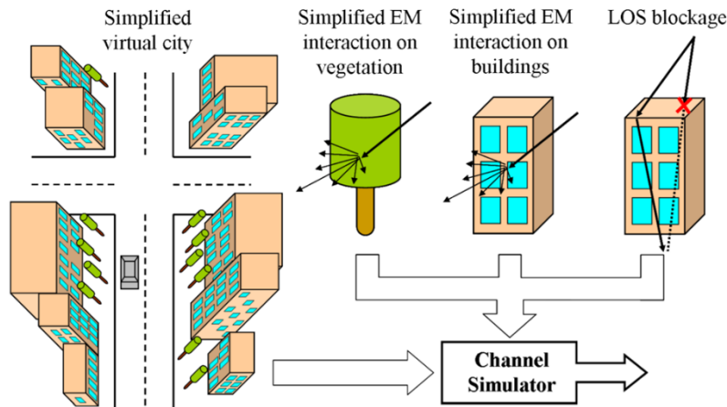
Figure 2.18 – SCHUN macro architecture – source [22]
