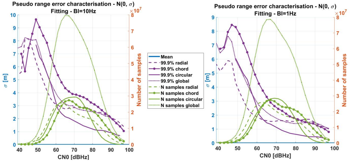
Figure 6.25 – pseudo range error characterization – Cases 1 to 4 – fitting – focus on 99.9% confidence level
