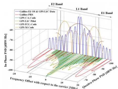
Figure 2.14 – Spectra of GPS and Galileo signals in L1 – source [19]
