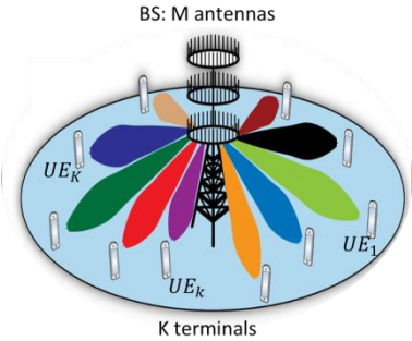
Figure 3.7 – massive MIMO model
