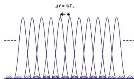
Figure 3.13 – OFDM subcarrier spacing
