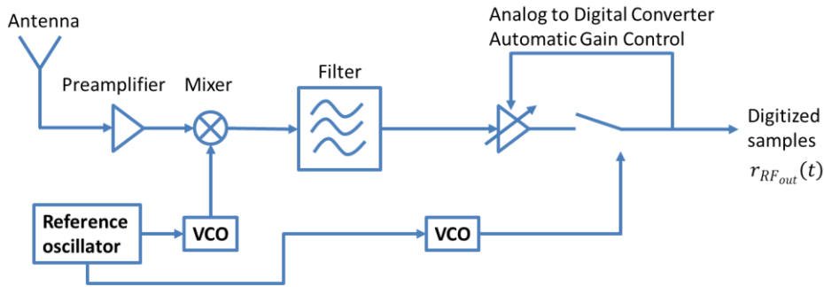
Figure 2.19 – Radio Frequency Front End
