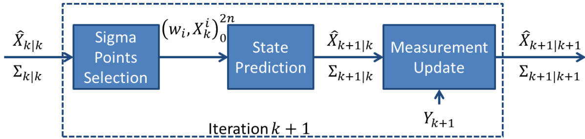
Figure 7.3 – UKF principle
