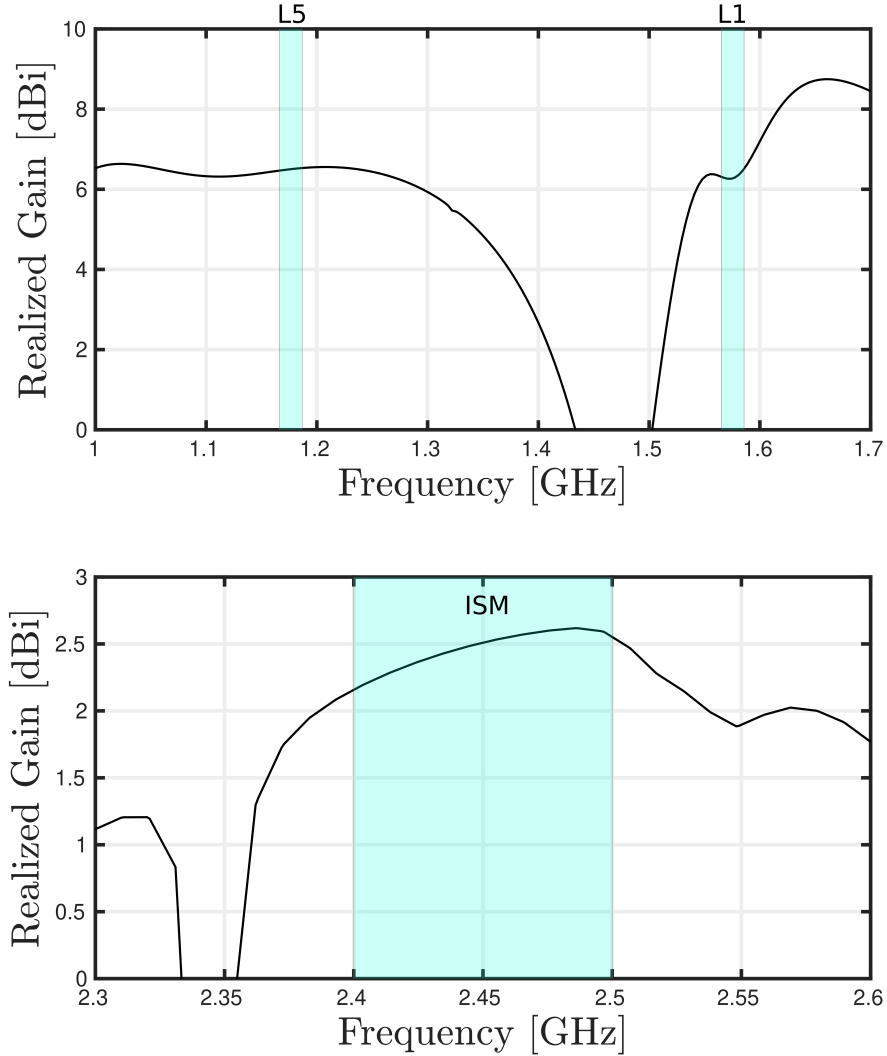
Figure 6.11: Simulated realized gain of the triple-band DRA at the (a) GNSS, for \theta = 0^\circ and \phi = 0^\circ , and (b) ISM, for \theta = 60^\circ and \phi = 0^\circ , bands.
