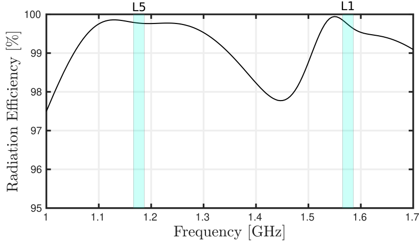
Figure 3.18: Simulated radiation efficiency of the proposed DRA.
