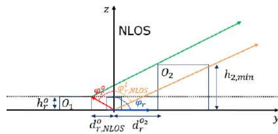
Figure 4-32– Scenario 2, y-z plane, NLOS reception state
