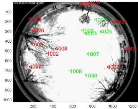
Figure 5-23 – Possible image processing NLOS/LOS estimation: the green points are considered in the sky-area, the red points are considered to be obstructed by obstacles
