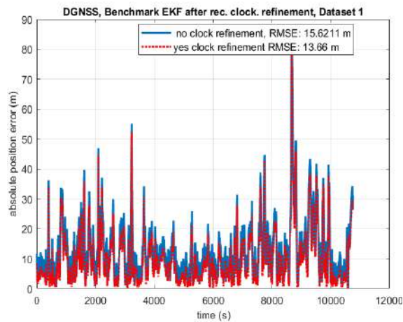
Figure 7-20 – Absolute Position estimation error with the corresponding RMSE: Dataset 1, DGNSS Benchmark EKF, without refined receiver clock model (blue line) vs. with refined receiver clock model (red line)
