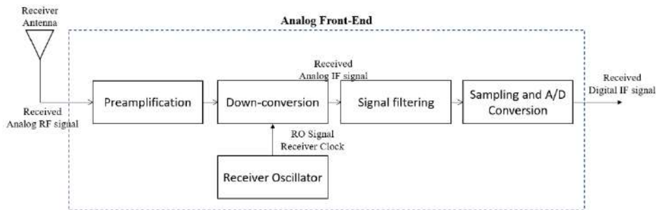
Figure 2-27 – Analog Front-end block scheme
