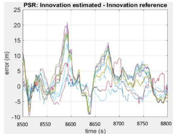
Figure 7-29 – Dataset 1, DGNS PVT solutions: Difference between Pseudorange EKF Innovations and Pseudorange Innovations obtained using reference SPAN positions, applying IF method
