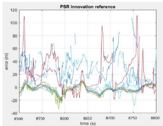
Figure 7-28 – Dataset 1, DGNS PVT solutions: Pseudorange Innovation values obtained using reference SPAN positions, applying IF method
