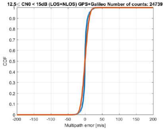
Figure 10-113 – Dual constellation PSR-R MN error CDFs for 12.5 \text{ dB-Hz} \leq C/N_0 < 15 \text{ dB-Hz} . In blue: original PSR-R MN error CDF. In red: Gaussian overbounding CDF
