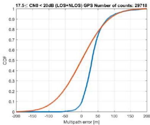
Figure 10-49 – GPS PSR MN error CDFs for 17.5 dB-Hz \leq C/N_0 < 20 dB-Hz. In blue: original PSR MN error CDF. In red: Gaussian overbounding CDF
