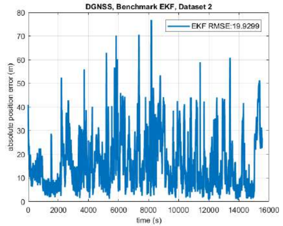
Figure 7-10 – Absolute Position estimation error with the corresponding RMSE: Dataset 2, DGNSS Benchmark EKF
