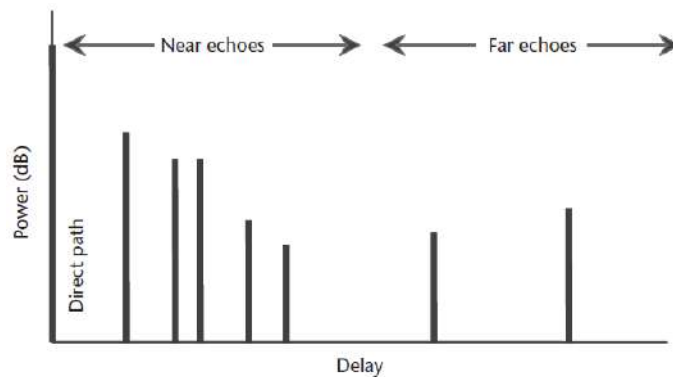
Figure 2-28 – Canonical power-delay-profile for land-mobile satellite channel [12]
