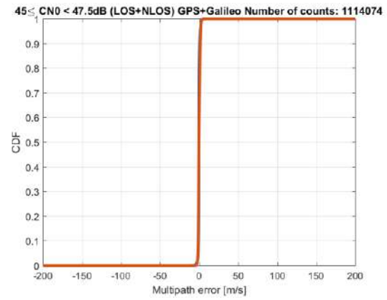
Figure 10-140 – Dual constellation PSR-R MN error CDFs for 45 dB-Hz C/N_0 < 47.5 dB-Hz. In blue: original PSR-R MN error CDF after mean removal application. In red: Gaussian overbounding CDF
