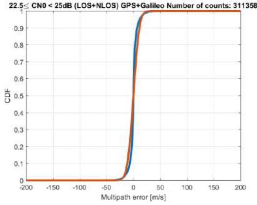
Figure 10-121 – Dual constellation PSR-R MN error CDFs for 22.5 \text{ dB-Hz} \leq C/N_0 < 25 \text{ dB-Hz} . In blue: original PSR-R MN error CDF. In red: Gaussian overbounding CDF
