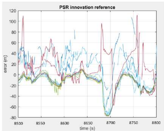
Figure 7-12 – Dataset 1, DGNSS Benchmark EKF: PSR Innovation values obtained using reference SPAN positions
