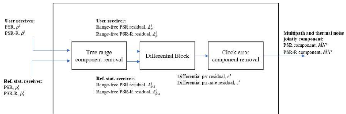
Figure 5-2 – Single Constellation MN Isolation Block
