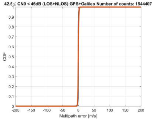
Figure 10-137 – Dual constellation PSR-R MN error CDFs for 42.5 dB-Hz \leq C/N_0 < 45 dB-Hz. In blue: original PSR-R MN error CDF. In red: Gaussian overbounding CDF
