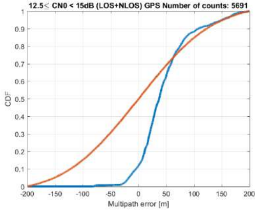
Figure 10-45 – GPS PSR MN error CDFs for 12.5 dB-Hz \leq C/N_0 < 15 dB-Hz. In blue: original PSR MN error CDF. In red: Gaussian overbounding CDF
