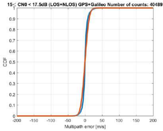
Figure 10-115 – Dual constellation PSR-R MN error CDFs for 15 \text{ dB-Hz} \leq C/N_0 < 17.5 \text{ dB-Hz} . In blue: original PSR-R MN error CDF. In red: Gaussian overbounding CDF
