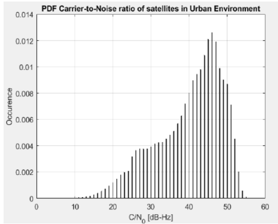
Figure 6-34 – Statistics of C/N_0 for dual constellation dataset
