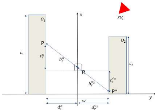
Figure 4-10 – Urban trench geometric model, x-y plane
