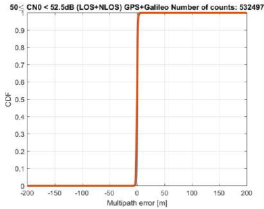
Figure 10-39 – Dual constellation PSR MN error CDFs for 50 \text{ dB-Hz} \leq C/N_0 < 52.5 \text{ dB-Hz} . In blue: original PSR MN error CDF. In red: Gaussian overbounding CDF
