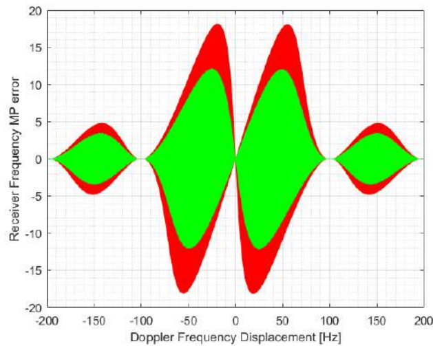
Figure 4-36 – Behavior of the Doppler frequency multipath error envelope (output of the FLL discriminator) affected by the presence of multipath ray, described by the MP-to-LOS power ratio, \alpha_1 , the Doppler Frequency Displacement \Delta D , and the Initial Phase Displacement \Delta\varphi .
