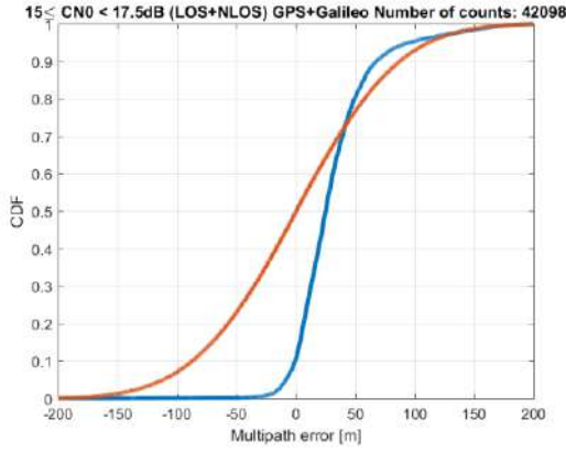
Figure 10-11 – Dual constellation PSR MN error CDFs for 15 \text{ dB-Hz} \leq C/N_0 < 17.5 \text{ dB-Hz} . In blue: original PSR MN error CDF. In red: Gaussian overbounding CDF
