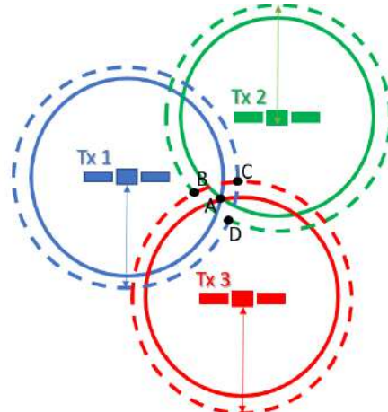
Figure 2-2 – Effect of receiver clock offset on GNSS-based Trilateration
