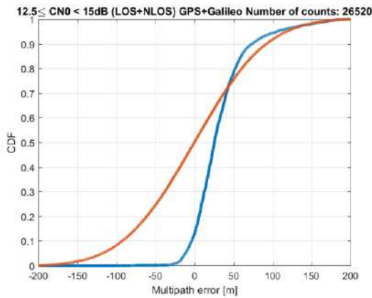
Figure 10-9 – Dual constellation PSR MN error CDFs for 12.5 \text{ dB-Hz} \leq C/N_0 < 15 \text{ dB-Hz} . In blue: original PSR MN error CDF. In red: Gaussian overbounding CDF
