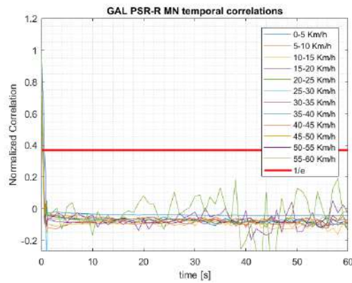
Figure 6-49 – One-dimension Time-Velocity Correlation of Galileo PSR-R MN residual error
