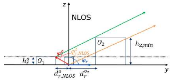
Figure 4-32– Scenario 2, y-z plane, NLOS reception state
