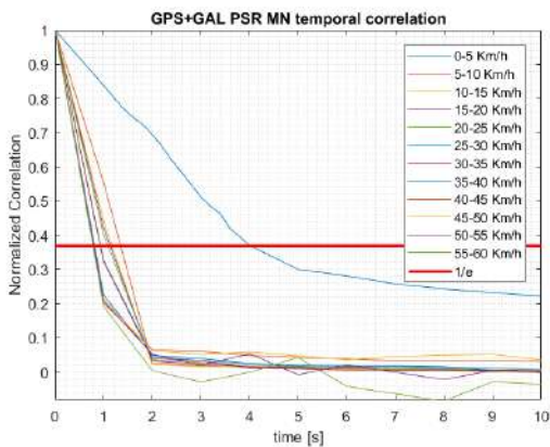
Figure 6-45 – Zoom of Figure 6-44 around 1/e cross-point
