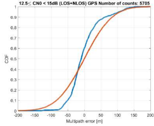
Figure 10-46 – GPS PSR MN error CDFs for 12.5 dB-Hz \leq C/N_0 < 15 dB-Hz. In blue: original PSR MN error CDF after mean removal application. In red: Gaussian overbounding CDF
