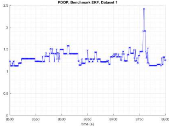
Figure 7-14 – PDOP values of DGNSS Benchmark EKF, applied to Data Collection 1, in the temporal section presented in Figure 7-11
