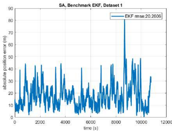
Figure 7-7 – Absolute Position estimation error with the corresponding RMSE: Dataset 1, SA Benchmark EKF
