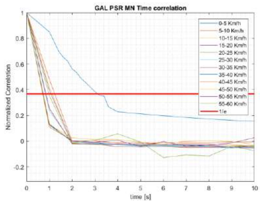
Figure 6-43 – Zoom of Figure 6-42 around 1/e cross-point
