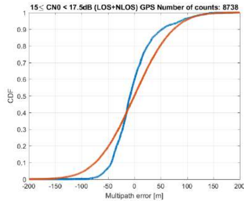
Figure 10-48 – GPS PSR MN error CDFs for 15 dB-Hz \leq C/N_0 < 17.5 dB-Hz. In blue: original PSR MN error CDF after mean removal application. In red: Gaussian overbounding CDF
