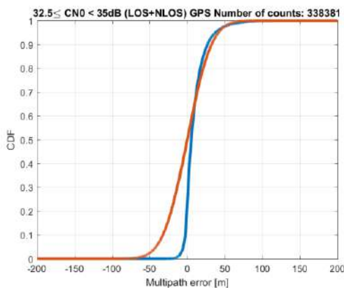
Figure 10-61 – GPS PSR MN error CDFs for 32.5 \text{ dB-Hz} \leq C/N_0 < 35 \text{ dB-Hz} . In blue: original PSR MN error CDF. In red: Gaussian overbounding CDF
