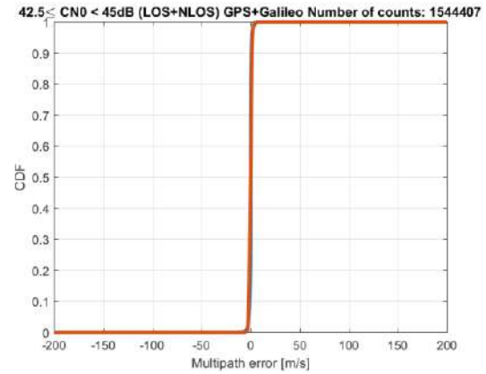
Figure 10-138 – Dual constellation PSR-R MN error CDFs for 42.5 dB-Hz \leq C/N_0 < 45 dB-Hz. In blue: original PSR-R MN error CDF after mean removal application. In red: Gaussian overbounding CDF
