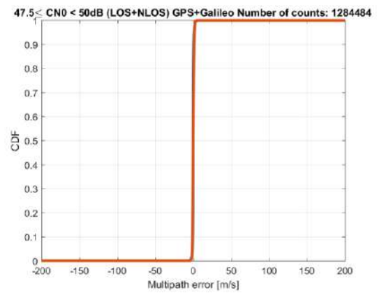
Figure 10-142 – Dual constellation PSR-R MN error CDFs for 47.5 dB-Hz C/N_0 < 50 dB-Hz. In blue: original PSR-R MN error CDF after mean removal application. In red: Gaussian overbounding CDF
