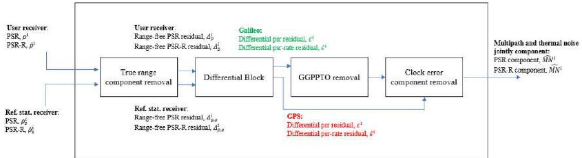
Figure 5-7 – Dual Constellation MN Isolation Block
