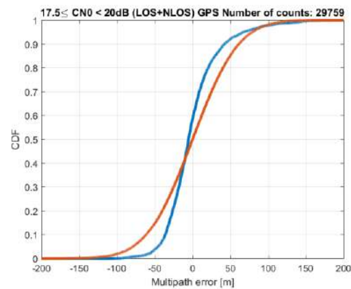
Figure 10-50 – GPS PSR MN error CDFs for 17.5 dB-Hz \leq C/N_0 < 20 dB-Hz. In blue: original PSR MN error CDF after mean removal application. In red: Gaussian overbounding CDF
