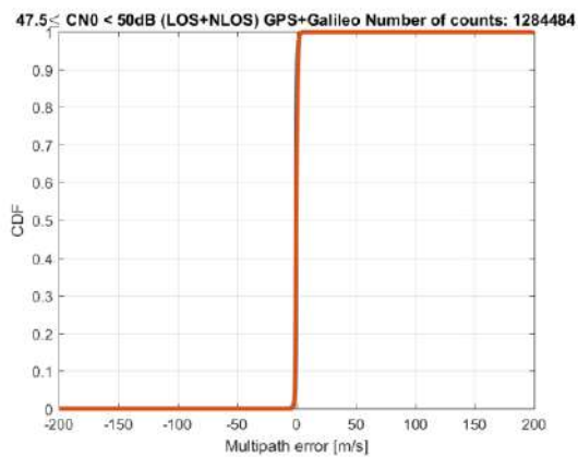
Figure 10-141 – Dual constellation PSR-R MN error CDFs for 47.5 dB-Hz C/N_0 < 50 dB-Hz. In blue: original PSR-R MN error CDF. In red: Gaussian overbounding CDF
