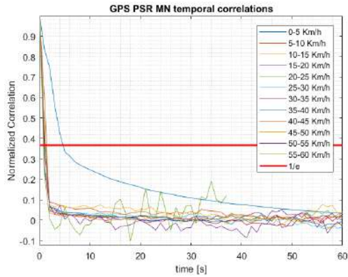
Figure 6-40 – One-dimension Time-Velocity Correlation of GPS PSR MN error residuals
