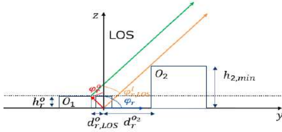
Figure 4-31 – Scenario 2, y-z plane, LOS reception state
