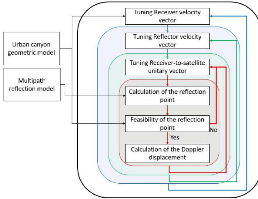
Figure 4-21 – Simulation of Doppler frequency displacement, algorithm's steps
