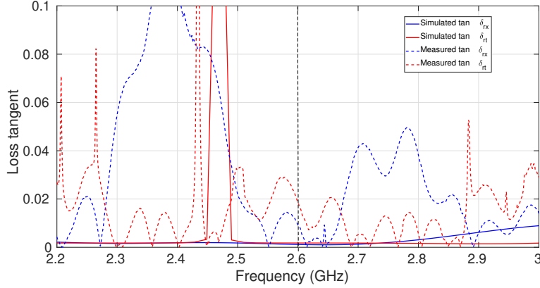
Figure 3.32: Simulated and measured loss tangent of the uniaxial anisotropic dielectric sample.
