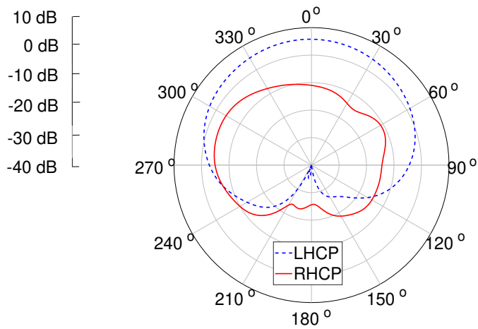
(a) RHCP and LHCP gain considering \phi = 0^\circ .
