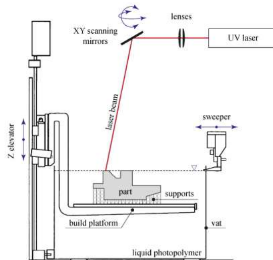
Figure 3.1: Stereolithography setup [88].
