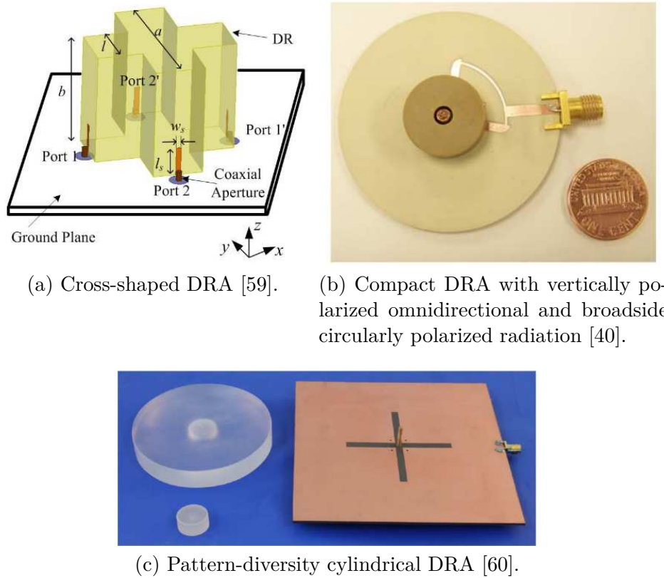
Figure 1.12: DRAs for multiband and pattern diversity applications.
