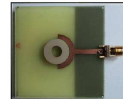
(b) Ring DRA with annular-shaped microstrip feed [51].
