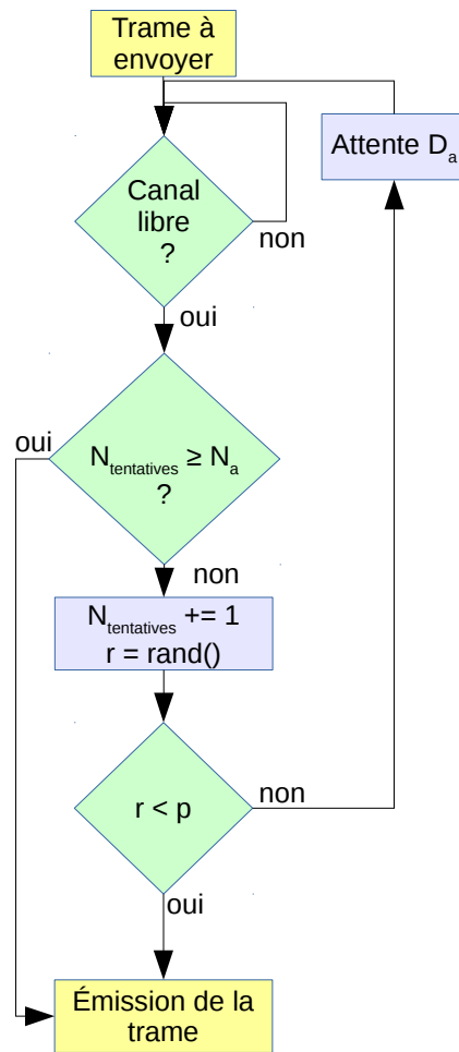
FIGURE 2.5 – Algorithme du CSMA p-persistent
