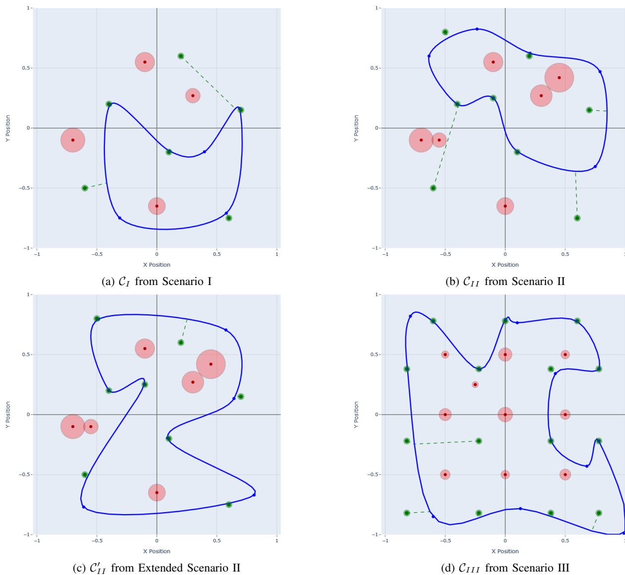
Fig. 6. Airspace corridors generated by the SMA for each scenario, corresponding to the highest scoring iterations discussed in Sec.IV-B1.
