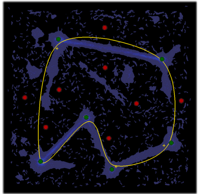
Fig. 1. Slime Mold Algorithm used for generating a corridor connecting vertiports (in green) while avoiding no fly zones (in red). The blue distribution is the pheromone grid, the media used by all the slime agents to communicate. They deposit pheromone to make a global distribution they can follow to reach all interest points.
