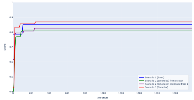
Fig. 5. Evolution of the global score R_{\text{global}} of the SMA generating \mathcal{C}_I , \mathcal{C}_{II} , and \mathcal{C}_{III} for the respective scenarios.
