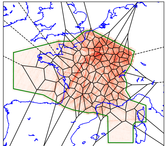
Fig. 14. Results with the non-linear dynamical system metric (NLDS) and \lambda = 0.4 .
