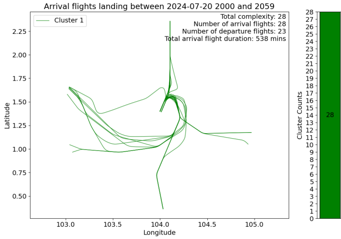
(a) This scenario shows the highest number of arrival flights where all trajectories fall into cluster 1.
