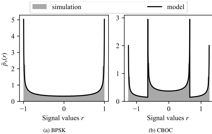
Figure 6: Single PRN GNSS signal distribution.
