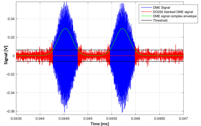
Fig. 2. Illustration of the RTCA DO-292 instantaneous blander behavior over the DME signal.
