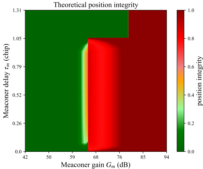
Figure 13: Theoretical position integrity under onboard meaconing, depending on G_m and \tau_m .
