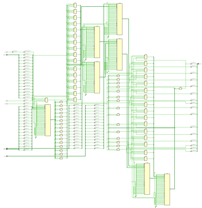
Fig. 17: PI controller circuit
