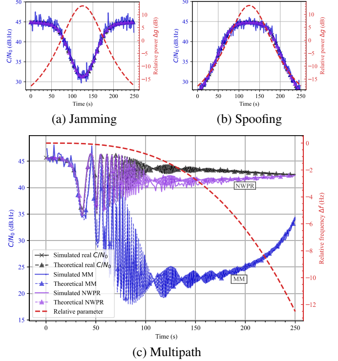
Fig. 1. Comparison between simulated C/N_0 results and presented models (legend shared between subFigs.)
