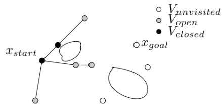
(d) All neighbors of z are visited and are added to V_{open} . z is added to V_{closed} . FMT* moves to the next iteration with the node which has the lowest cost.
