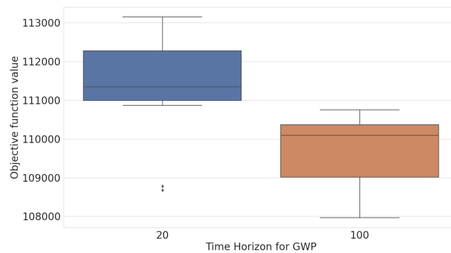
Figure 9: Distribution of the value of the objective function for the Paris-Miami tests, depending on the time horizon chosen for the GWP metric.
