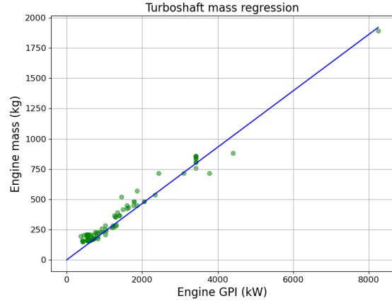
Fig. 4 Correlation between GPI and turboshaft mass
