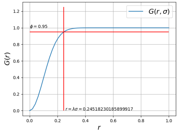
(b) Newton's method to determine r = \mathcal{G}_H^{-1}(\varphi) .
