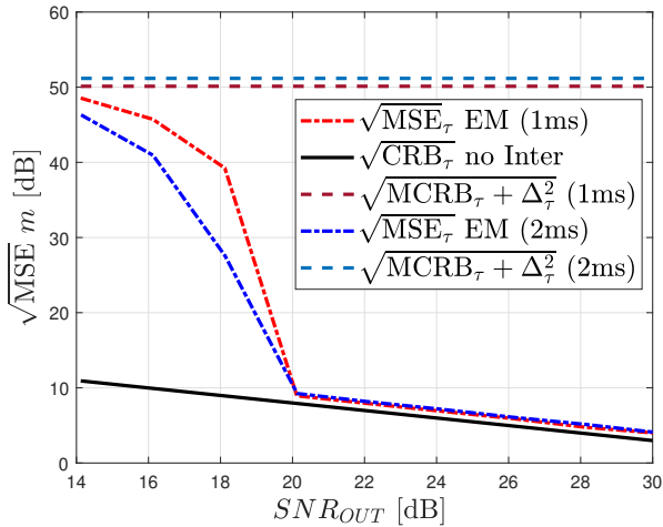
Fig. 1. EM algorithm estimator RMSE for time-delay of the GPS L1 C/A signal received along with a centered chirp signal of bandwidth B_c = 2 MHz and amplitude A = 40 . The sampling frequency is set to F_s = 4 MHz.
