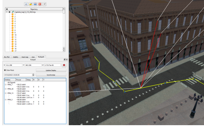
Figure 6: Capitole place (Toulouse center) multipath environment, SE-Nav software
