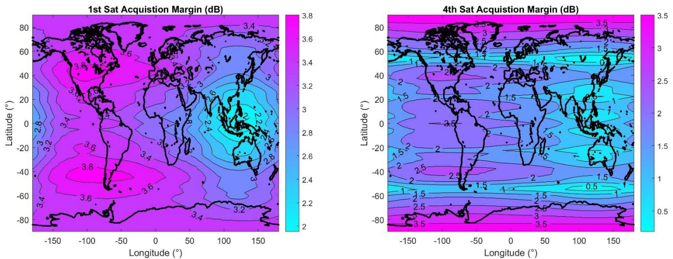
Figure 13 Acquisition C/N_0 link budget margin for GPS L1C/A signal
