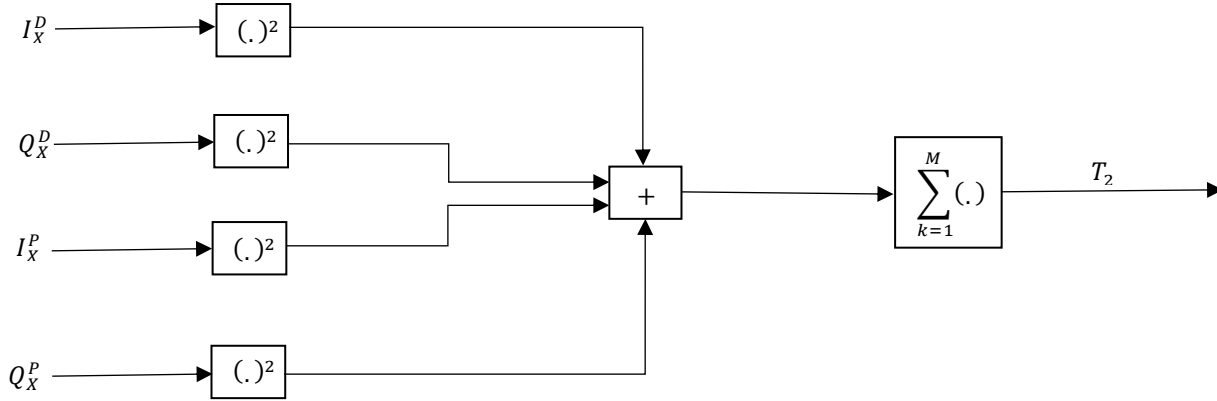
Figure 6 Acquisition detector for two components GNSS signal
