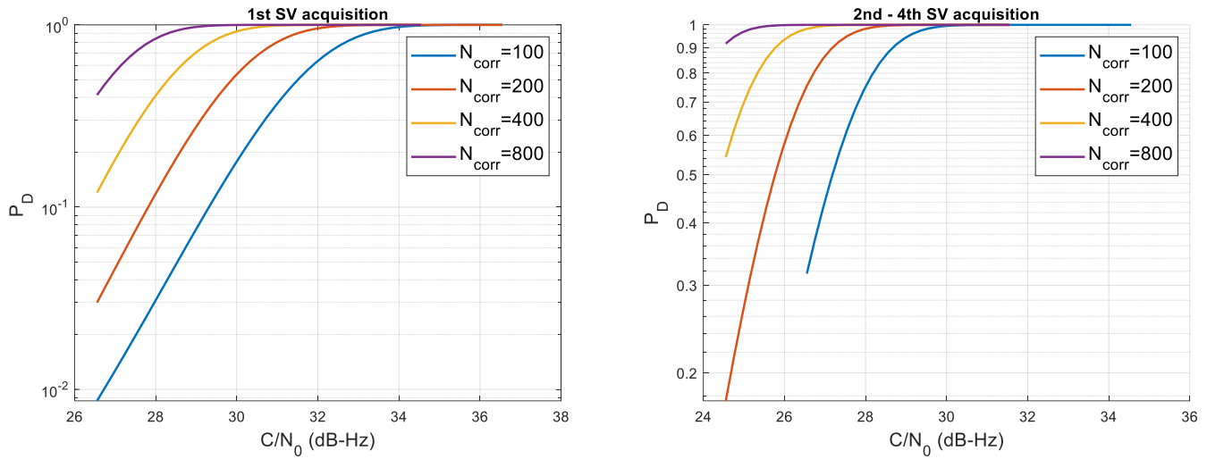
Figure 9 Probability of detection for GPS L5 and Galileo E5a SVs
