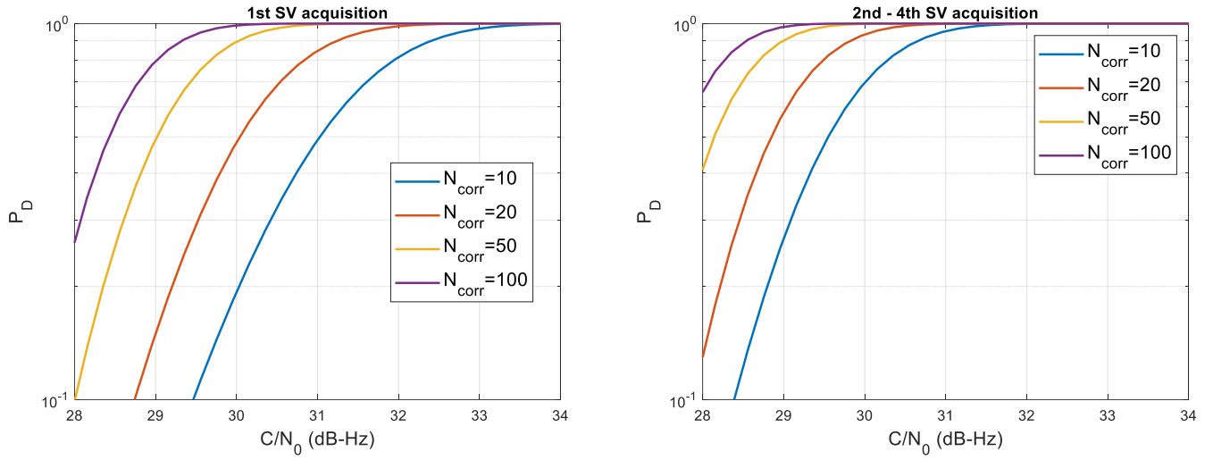
Figure 7 Probability of detection for GPS L1C/A SVs
