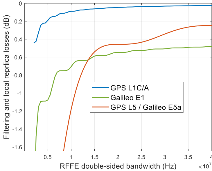
Figure 4 Band-limiting and local replica mismatch losses as a function of double-sided RFFE bandwidth
