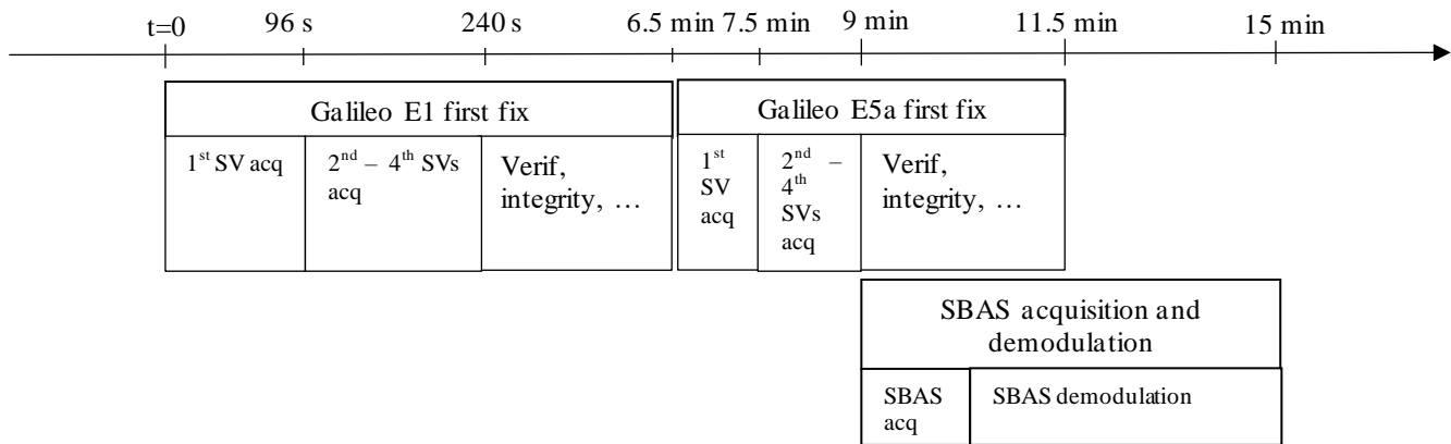
Figure 2 Galileo Acquisition Strategy Compliant with DMS:210
