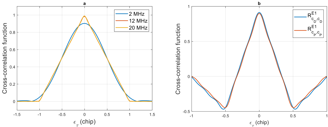
Figure 3 Impact of RFFE bandwidth on correlation function
