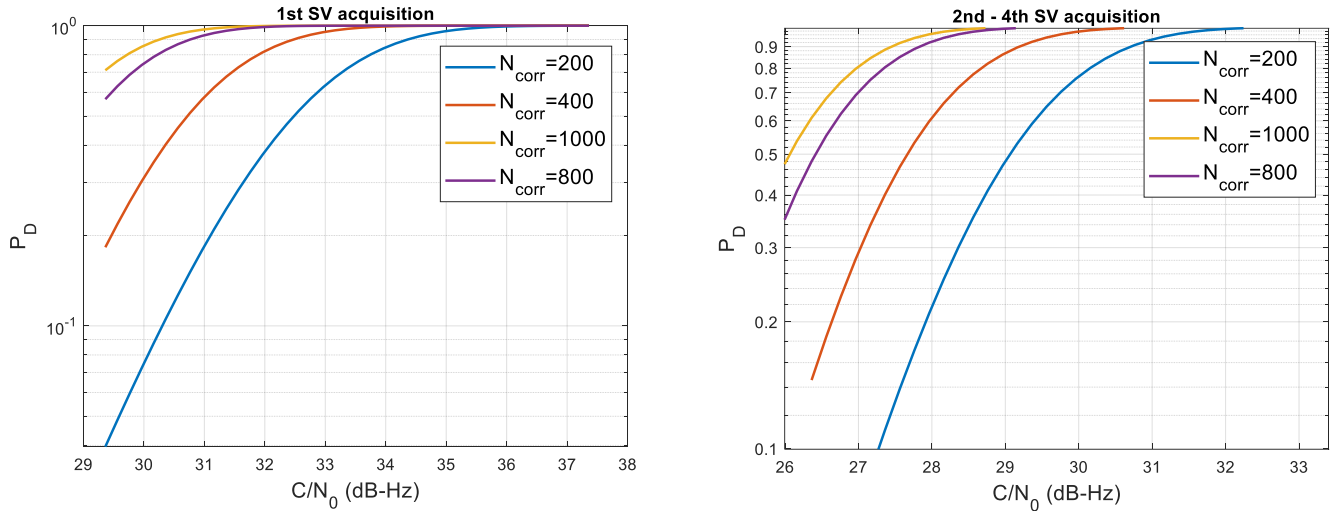
Figure 8 Probability of detection for Galileo E1 SVs
