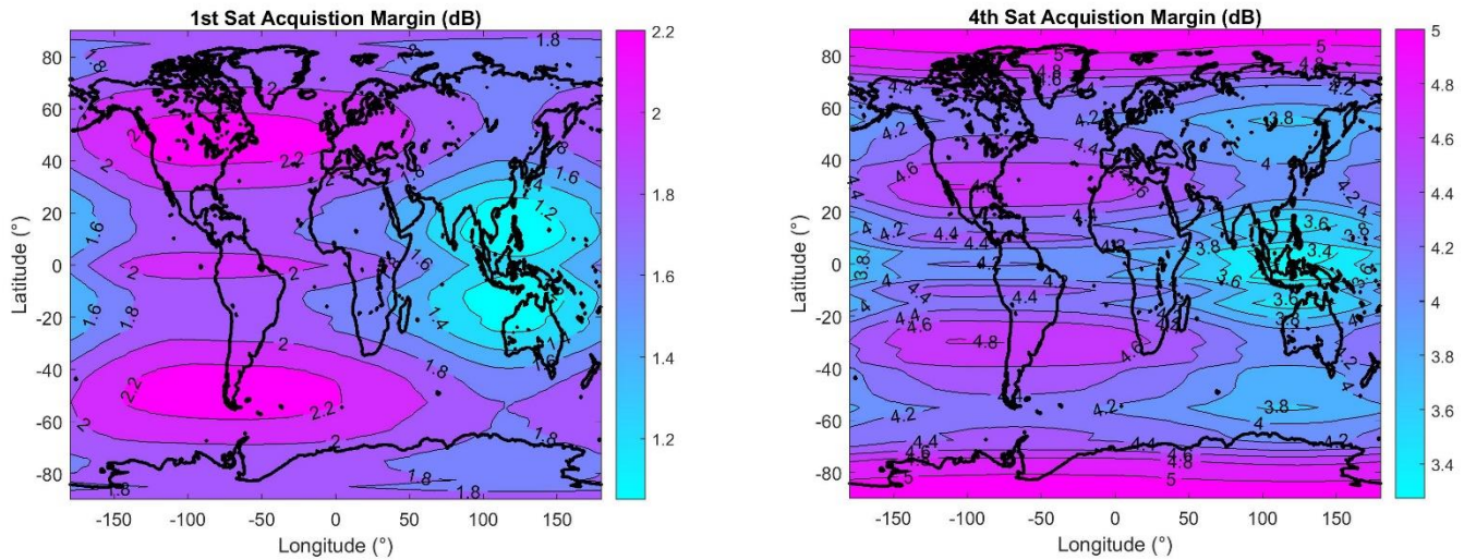
Figure 14 Acquisition C/N_0 link budget margin for Galileo E1 signal
