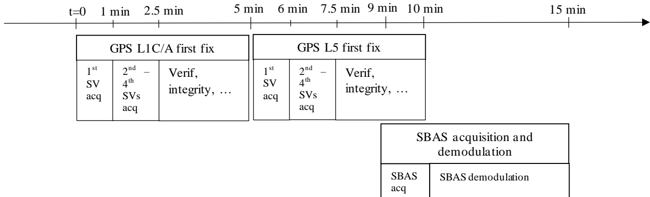
Figure 1 GPS Acquisition Strategy Compliant with DMS:199
