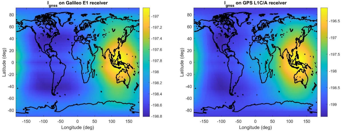
Figure 12 I_{gnss} on Galileo E1 and GPS L1C/A receiver
