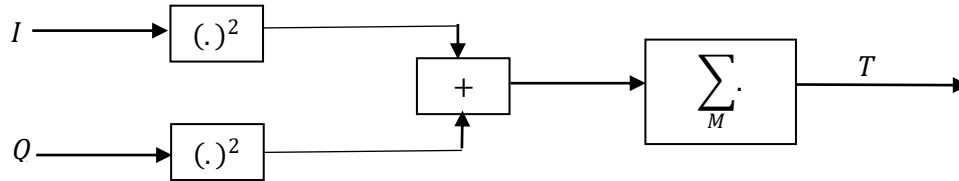
Figure 5 One GNSS component acquisition detector
