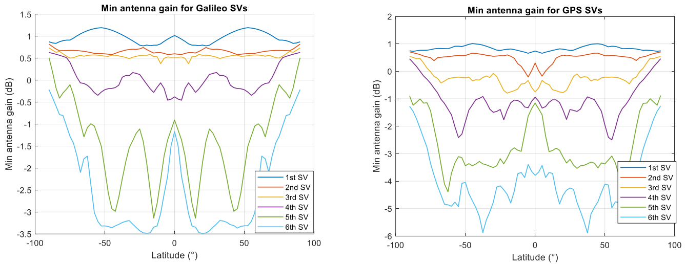
Figure 11 Minimum antenna gain
