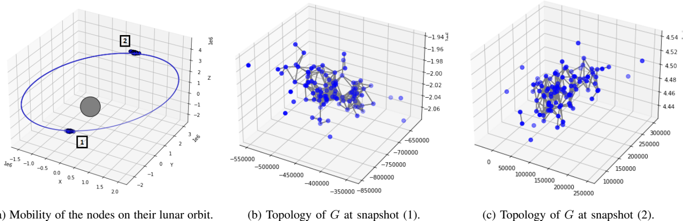
Fig. 2: Dynamic topology of graph G . The orbit of G is defined as the average orbit of its |N| nodes. Each node position is derived with a random offset to the first node position, which is fixed (see Section III-A).
