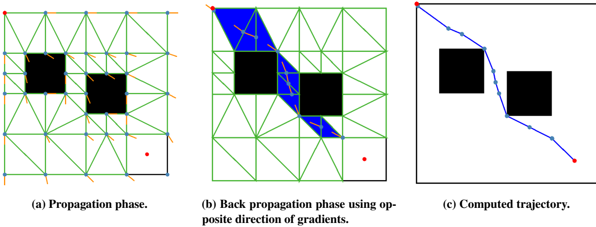
Fig. 8 Optimal trajectory generation with the Fast Marching algorithm. Gradients are represented in orange, mesh nodes in blue, and mesh triangles in green.
