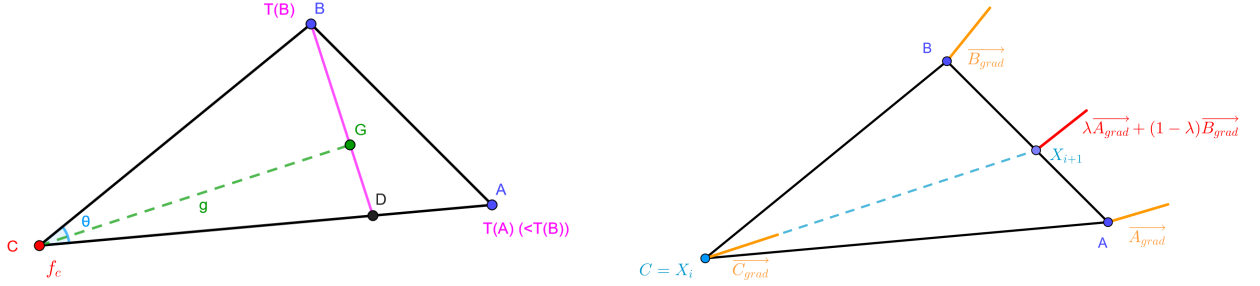
(a) Update on a triangle: A, B and C are some of the vertices of the triangular mesh. \overrightarrow{GC} is the gradient associated with vertex C .
