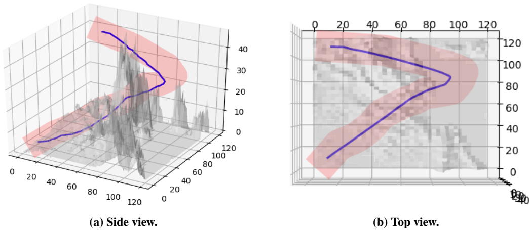
Fig. 30 Trajectory generated in an ANSA scenario with the Fast Marching algorithm (arb. unit).
