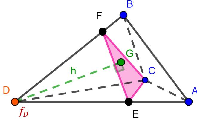
Fig. 18 Update on a tetrahedron: A, B, C and D are some of the vertices of the tetrahedral mesh. \overrightarrow{GD} is the gradient associated with vertex D.
