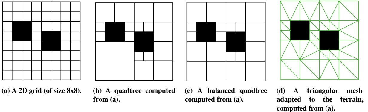
Fig. 5 Refinement of the data structure modeling a two-dimensional space.
