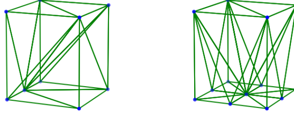
Fig. 15 Respectively, from left to right, templates with smaller neighbors in one inter-cardinal direction and in one cardinal direction.
