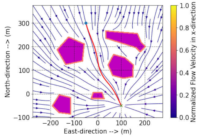
(b) Streamlines and path of vehicle 2.
