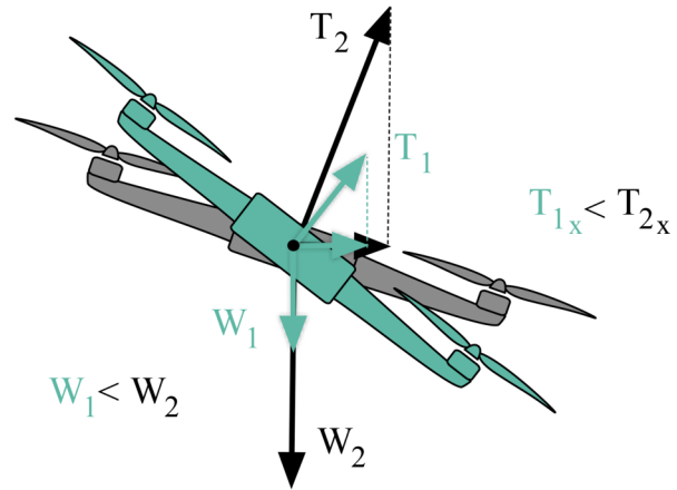
Figure 5. Thrust and weight forces applied on a quadrotor with two different masses. When the mass increases, the thrust increases to compensate for the weight, and the drag is also increased due to the increased motor speed, however, the overall bank angle is reduced.
