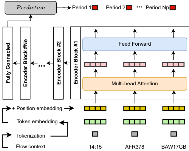
Figure 3: Proposed flow prediction model based on transformer neural networks.
