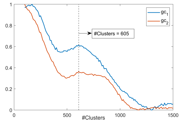
Figure 5: cluster Number determination.
