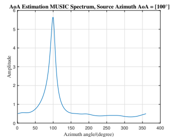
Figure 13. AoA estimation with 3D-VA at 100°.
