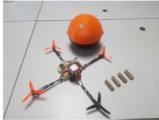
Figure 1: Quadrotor with additional masses and custom spherical body.
