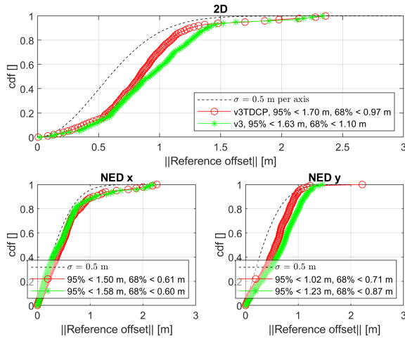
Figure 7: Highway CDFs.
