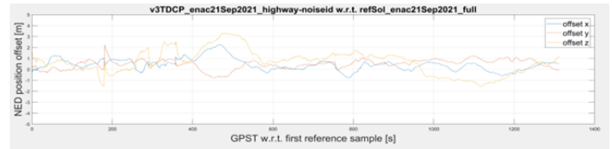
Figure 8: Highway Time series v3TDCP.
