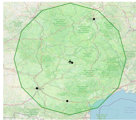
Fig. 7. Range and potential landing sites for TEFO situation
