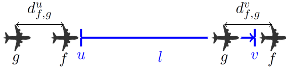
Fig. 4. Link conflict detection based on the comparison of distance between aircraft at the beginning or the end of a link with the separation minima
