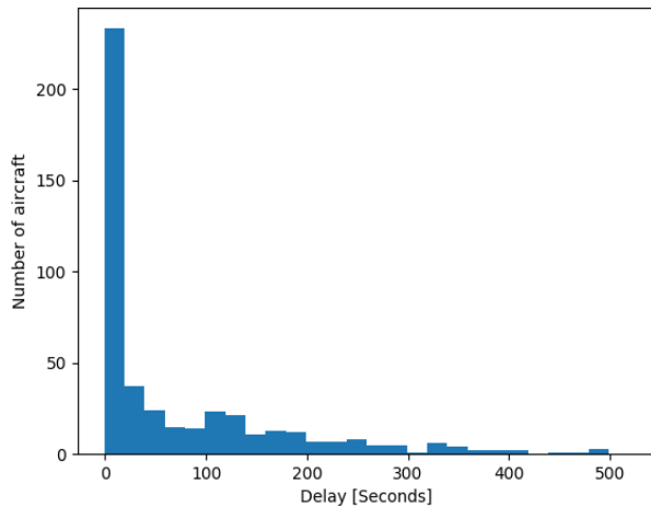
Fig. 11. Histogram representing the delay of aircraft in the scenario (687 aircraft)
