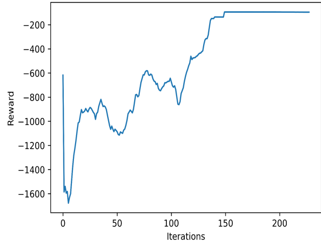
Fig. 9. Evolution of the total reward (sum of all aircraft's reward) of a given Sliding Window, this could be seen as the learning curve of the algorithm over a certain sliding window
