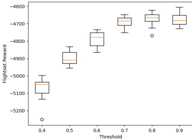
Fig. 7. Genetic algorithm results on critical flight set threshold parameter, 150 individuals evaluated over 10 generations
