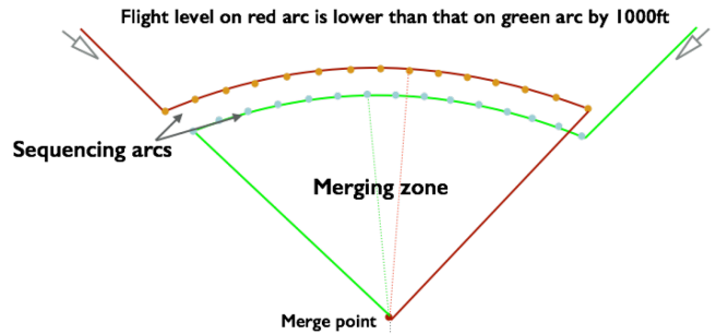
Fig. 2. Merge Point Topology : for each aircraft, the length of the flown sequencing arc is a decision variable
