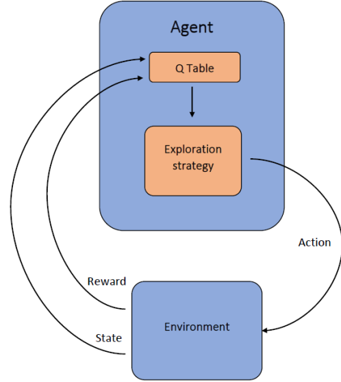
Fig. 3. The agent - environment interaction in a Q-Learning : the agent does not know his environment but only the state and reward following an action
