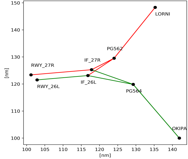
Fig. 1. Simplified STAR model at CDG: aircraft enter at LORNI or OKIPA. Merge points are located on both IF_27R and IF_26L
