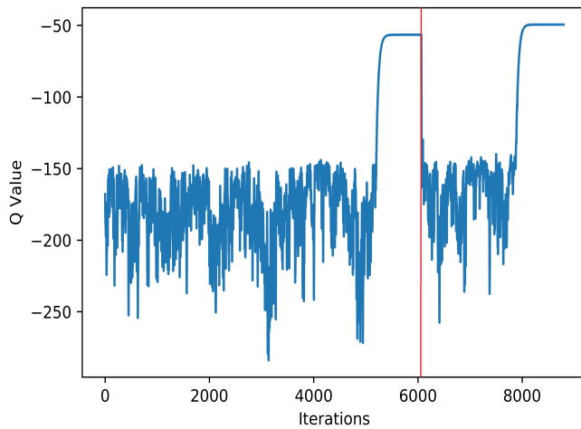
Fig. 8. Q value for a given aircraft over two sliding windows (separated with the red line).
