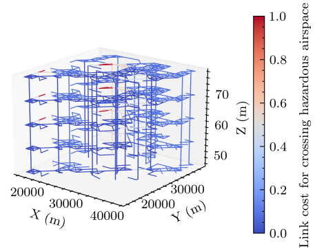
Figure 9: Normalized link cost for crossing hazardous airspace in route network
