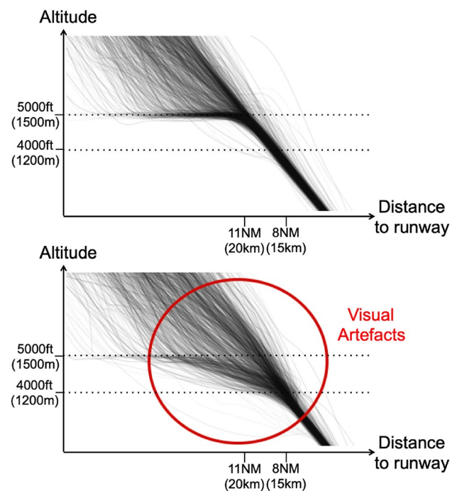
Fig. 4 This figure illustrates examples of good and poor usage of curve modifications for aircraft approach trajectory altitude profile. At the top, both the mean and the principal components were modified. At the bottom, only the mean was modified. The behavior observed while modifying only the mean curve presents artifacts. Level-off flight was expected, but the trajectories present descent phases. These behaviors are not nominal and underline that the process was not executed properly
