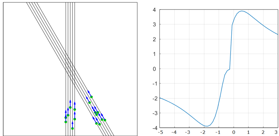
Figure 15. N-S and W-E flows crossing at 30 deg. Traffic situation on the left, complexity function of time on the right.
