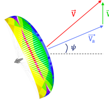
Fig. 4 Heading control
