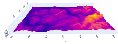
Fig. 3 Earth surface
