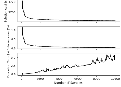
Fig. 10 Evolution of the solution with the number of samples.
