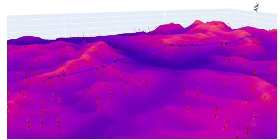
Fig. 15 3D plot of the computed trajectory for flight n°1, thermal areas are represented by red quivers.
