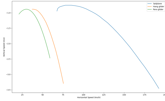
Fig. 6 Speed polar of soaring aircrafts
