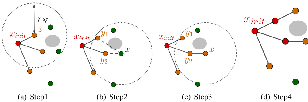
Fig. 7 One iteration of the FMT* algorithm.
