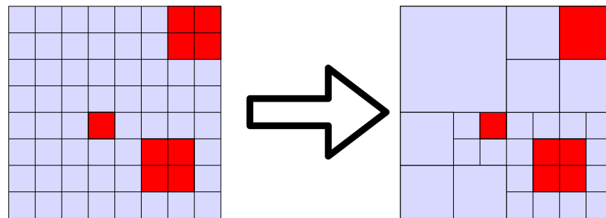
Figure 13. Example of a quadtree.
