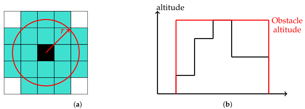
Figure 12. Enlargement of obstacles [7]. (a) Horizontal enlargement (obstacle cell: black, new obstacle cells: blue); (b) vertical enlargement.
