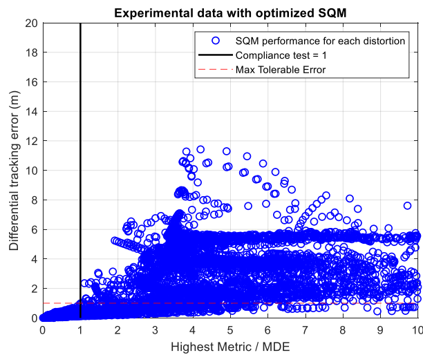
Figure 9 – SQM compliance prediction using experimental data and an optimized SQM algorithm
