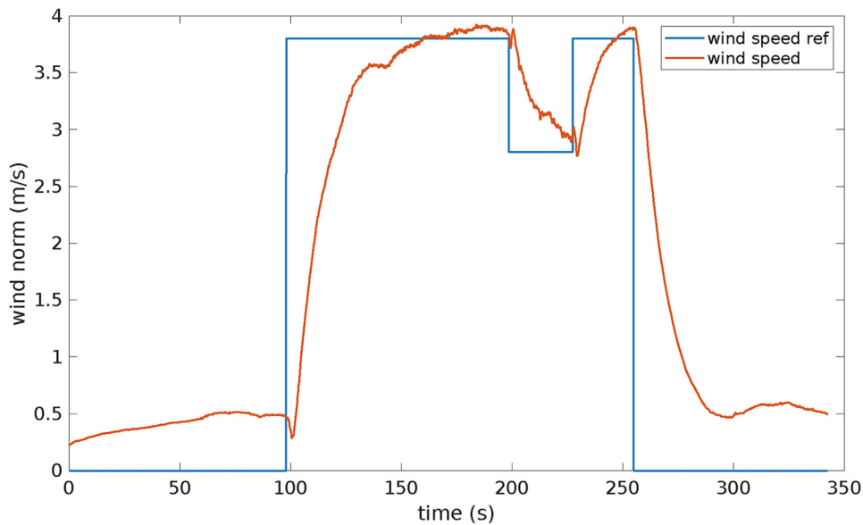
Figure 15. Evolution of the wind speed estimated from onboard filter and the reference wind speed.
