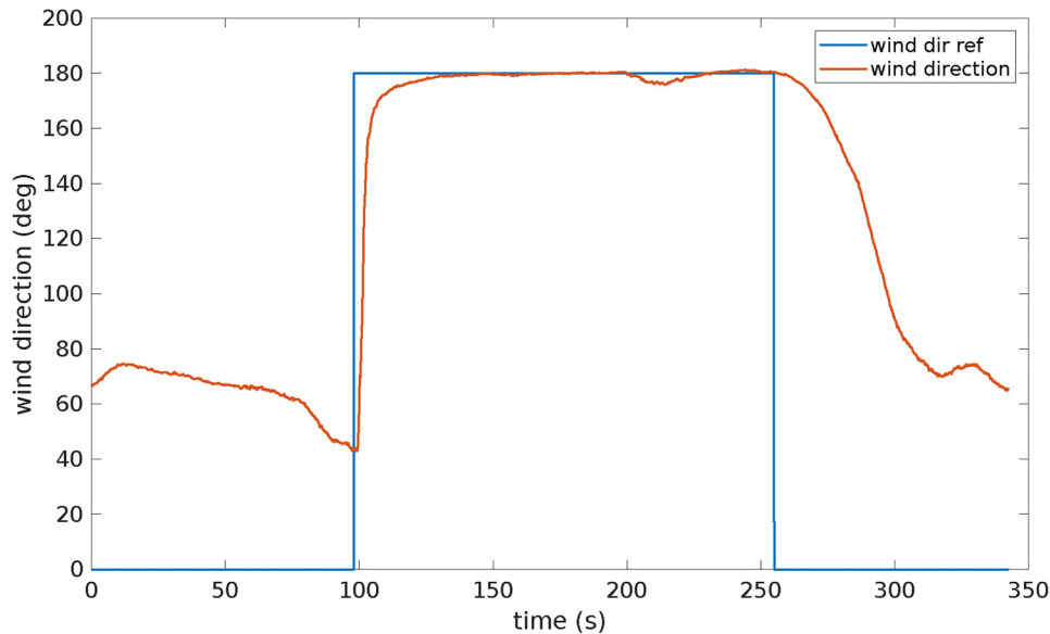
Figure 16. Evolution of the wind direction estimated from onboard filter and the reference wind direction.
