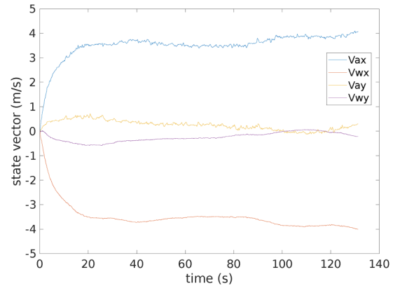
Figure 7. Evolution of the Kalman filter state vector over time during indoor flight.
