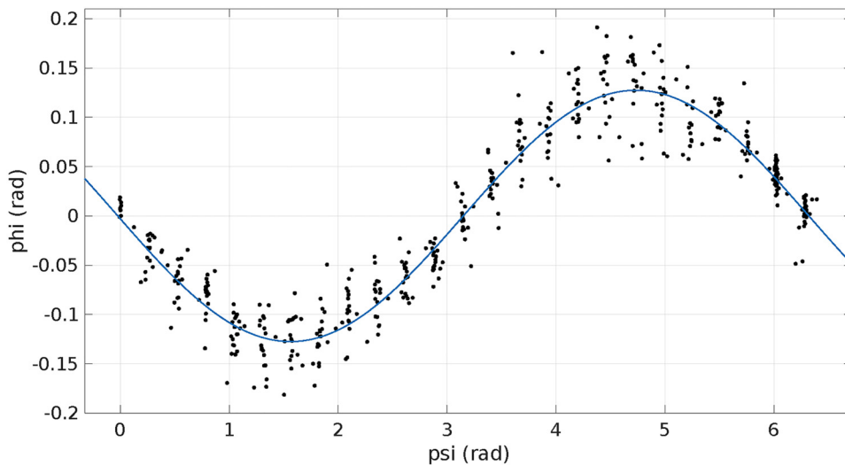
Figure 5. Roll angle \phi against heading angle \psi after a complete turn in from of the wind generator; the sinusoidal fitting curve is in blue.
