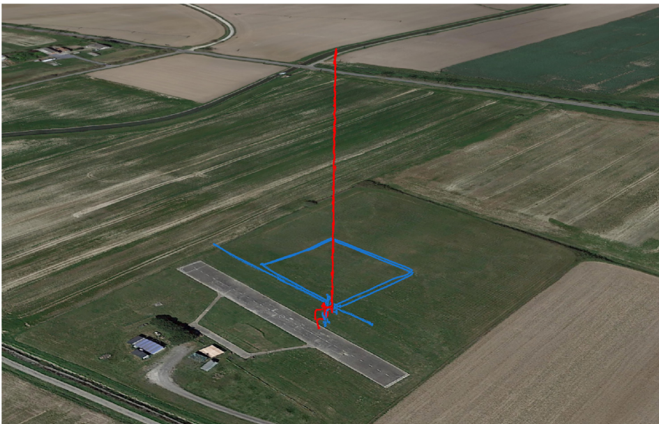
Figure 9. Trajectories for the outdoor flights: vertical profile in red, horizontal square at constant altitude in blue.
