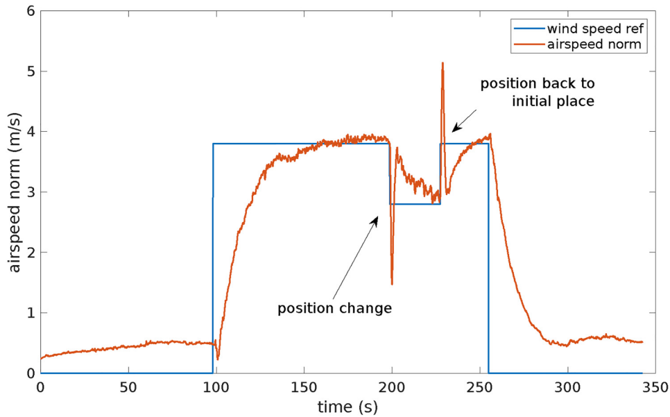
Figure 14. Evolution of the airspeed estimated from onboard filter and the reference wind speed.
