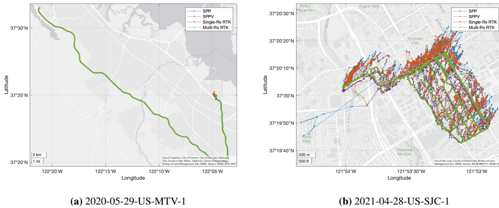
Figure 9: Estimated positions with SPP, SPPV, single-receiver RTK and multi-receiver RTK.
