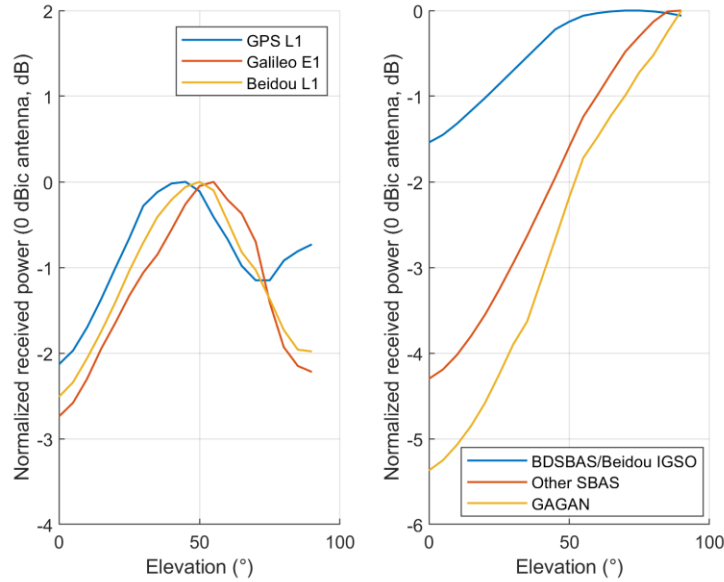
Figure 2: Transmit antenna gain and propagation attenuation pattern
