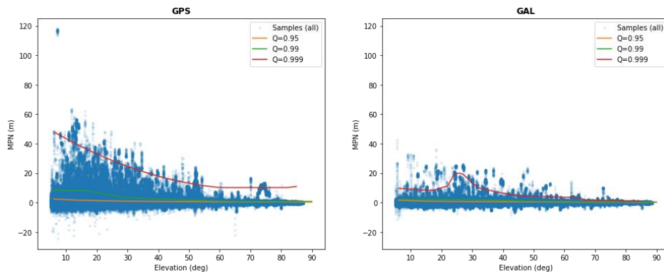
Figure 15 Multipath error modeling results with single feature (elevation) model
