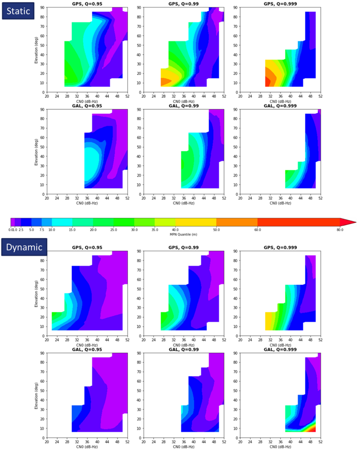
Figure 17 Multipath error modeling results with multiple feature (CNO and elevation) model for static (above) and dynamic (bottom) state
