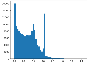
(b) with trajectory extension of p = 2 states before and after the reference state. No smoothing applied. 161,130 values with MAE = 0.3
