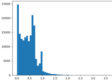
(a) with trajectory extension of p = 10 states before and after the reference state (to take into account uncertainty in the measurements). No smoothing applied. 182,982 non-zero values with MAE = 0.4
