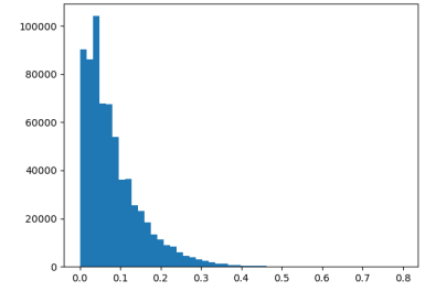
(c) with no trajectory extension and Gaussian smoothing. 678,240 values with MAE = 0.08
