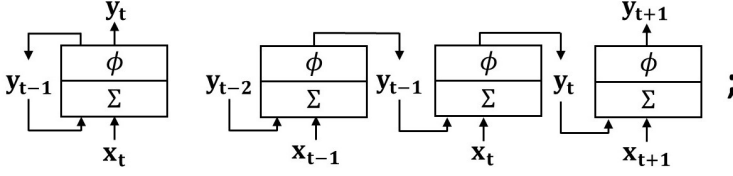
Figure 3: Basic RNN layer (left) and the same layer unrolled through time (right). \Sigma represents linear mapping and \phi represents the activation function.
