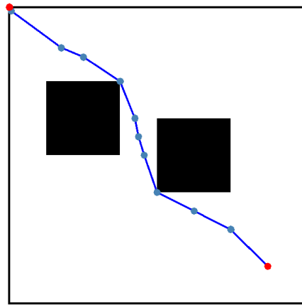
Figure 23: Trajectory generated with a Fast Marching algorithm on a 8 \times 8 grid. The trajectory generated is very close to the optimal path, with weak errors due to the discretization.
