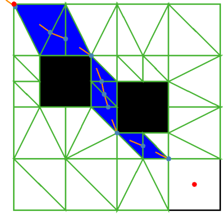
Figure 22: Back propagation from EndCoordinate . StartCoordinate (in the Northwest) and EndCoordinate (in the Southeast) are both represented in red, gradients in orange, mesh nodes in blue, and mesh triangles in green. Blue triangles are the triangles visited during back propagation.
