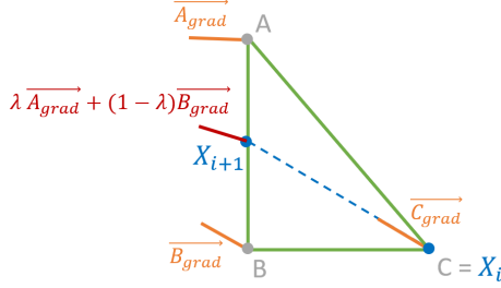
Figure 21: Interpolation of a gradient inside a triangle ABC. X_i is the last point visited by the back propagation. It coincides with the mesh vertex C , hence the gradient at X_i is \vec{C}_{grad} . The next point visited by the back propagation is X_{i+1} . It is at the intersection between \vec{C}_{grad} and the edge AB , hence the gradient has to be interpolated. The interpolation parameter is \lambda = \frac{\|\vec{X}_{i+1}\vec{B}\|}{\|\vec{AB}\|} . Thus, the gradient at X_{i+1} is \lambda\vec{A}_{grad} + (1-\lambda)\vec{B}_{grad} .
