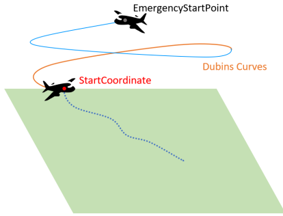
Figure 16: Initial procedure. From EmergencyStartPoint to StartCoordinate , if the generation of a single glide slope is impossible, the aircraft can make turns to lose altitude or get a better orientation.
