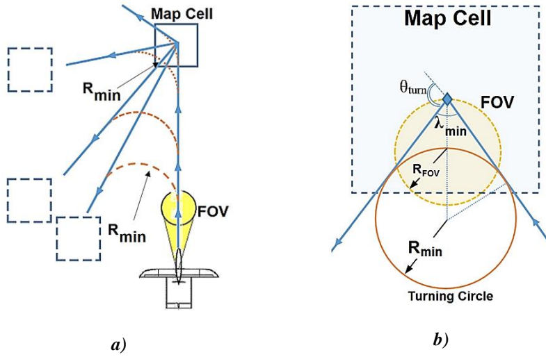
Fig. 2 Turning limitation. a) divers approaches to candidate cells with a minimum turn radius, b) maximum performance in turn due to cell coverage.
